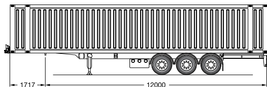
Conteneur 45'.
